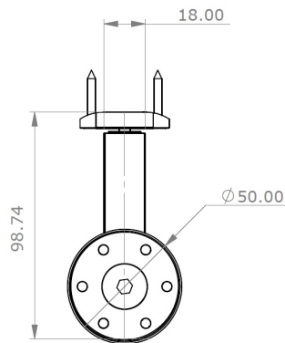
END VIEW
